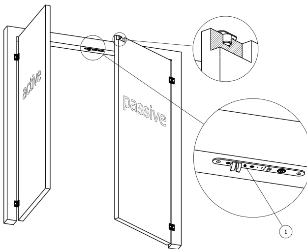
Automatic frame bolt – type 1 & 2
