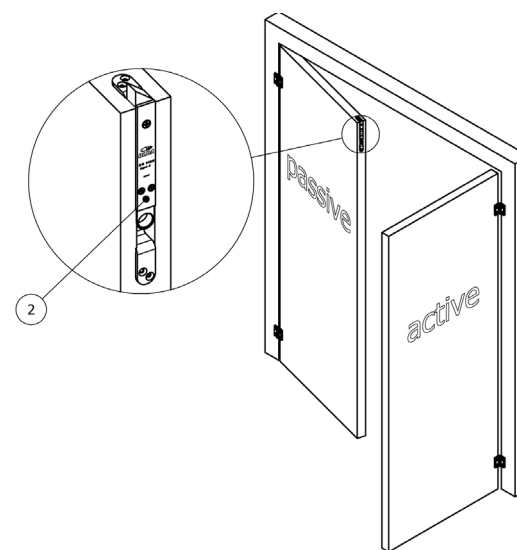
Semi-automatic flush bolt – type 1 & 2
