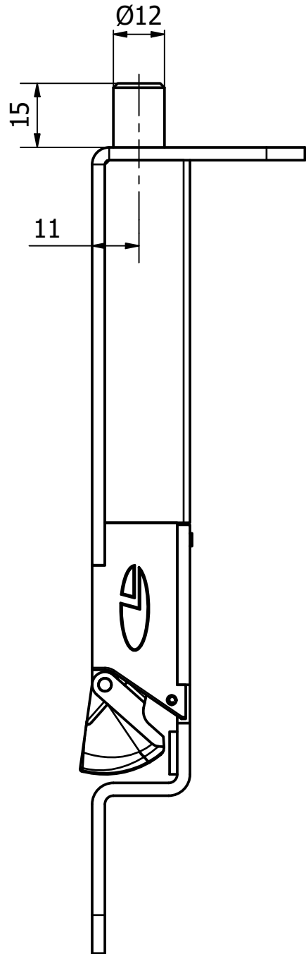
dimension drawing
